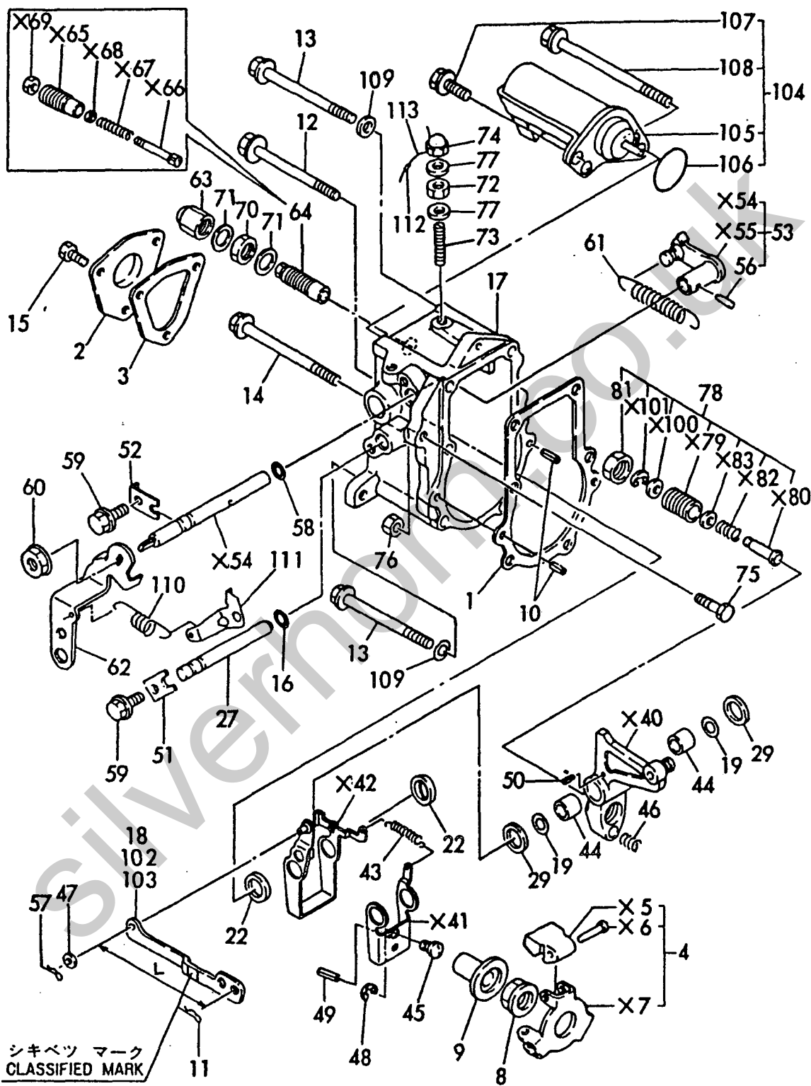
Fig. 12 ガバナ GOVERNOR
